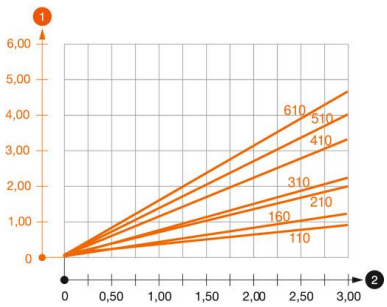
Diagramme de charge de la console AS 30
